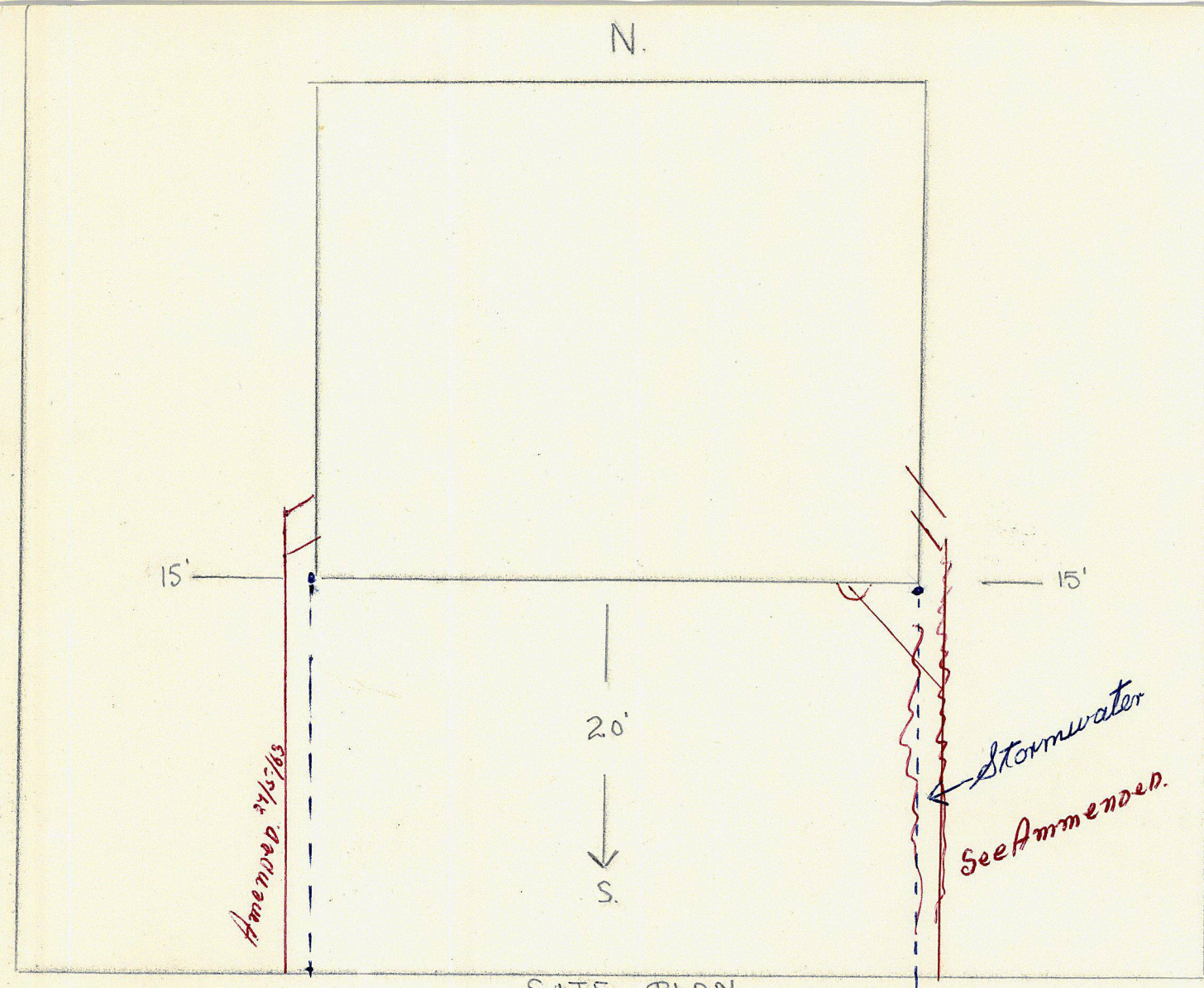
SITE PLAN, ROTHWELL STREET.
