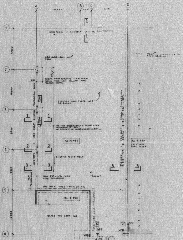
foundation plan
