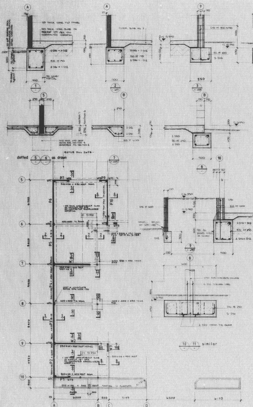
ground floor and foundation plan
