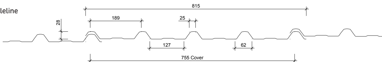
Veedek® (Formerly called Trimdek)
