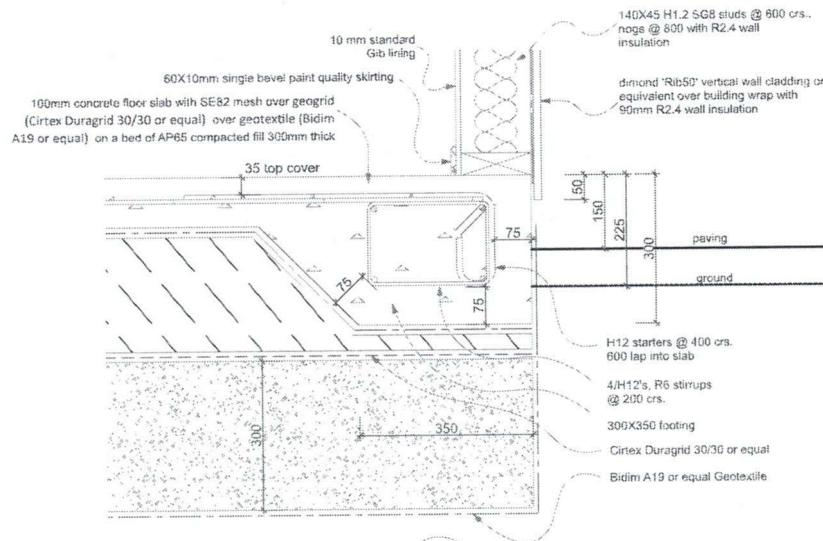
Grid 4 Slab Foundation Section Detail
