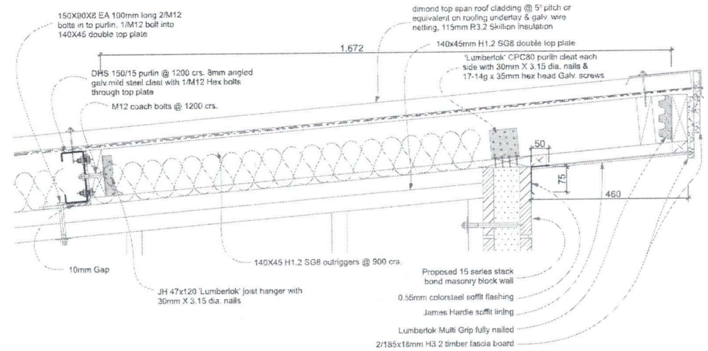
Grid C Outrigger connections Section Detail
