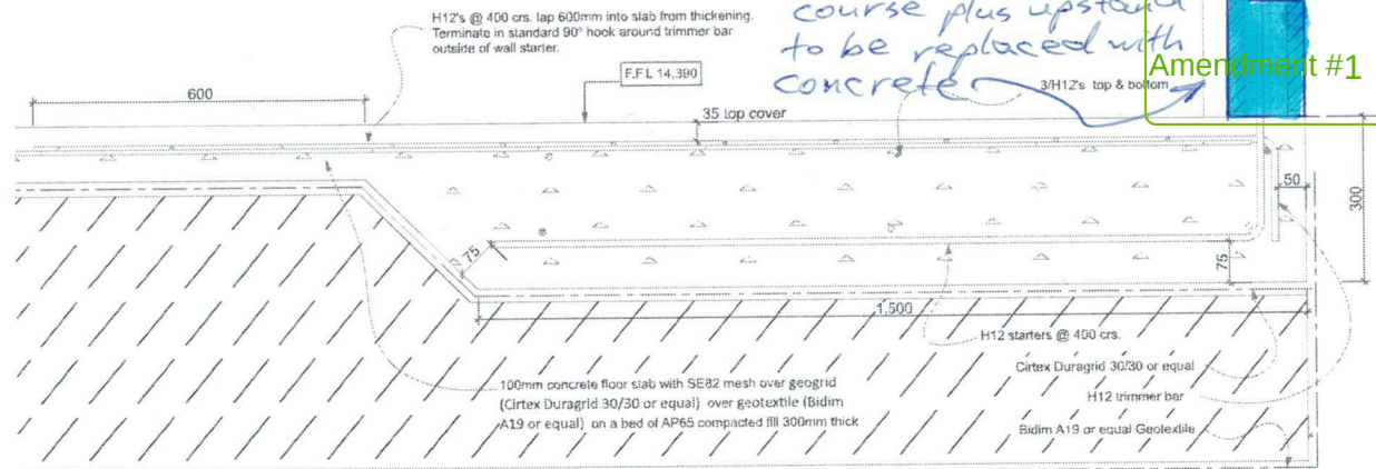
Grid C Slab Thickening Section Detail
