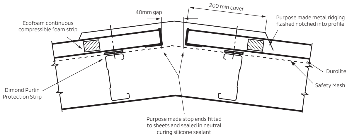
Fig 3 Detail At Ridge
