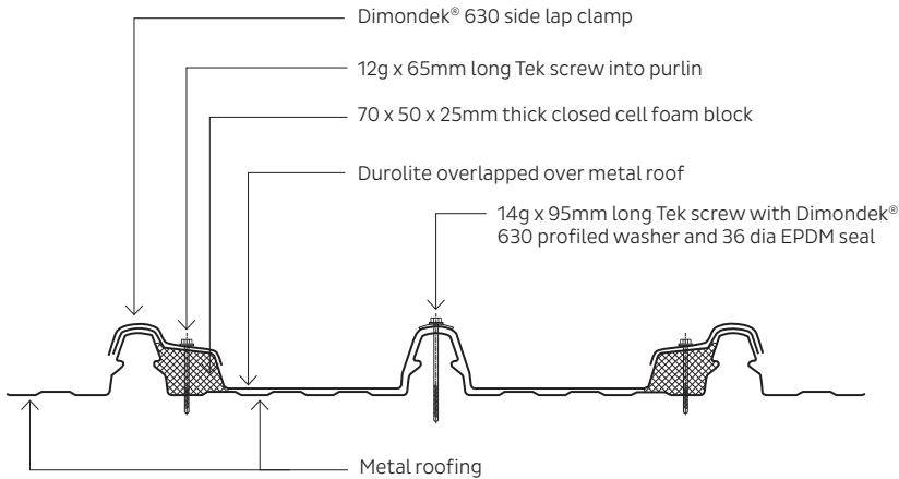
Fig 10 Durolite Dimondek® 630 Endlap Over Metal Roofing
