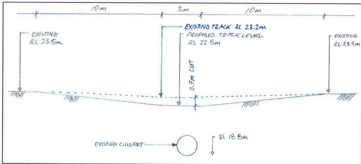
Figure 3 Proposed Track profile
