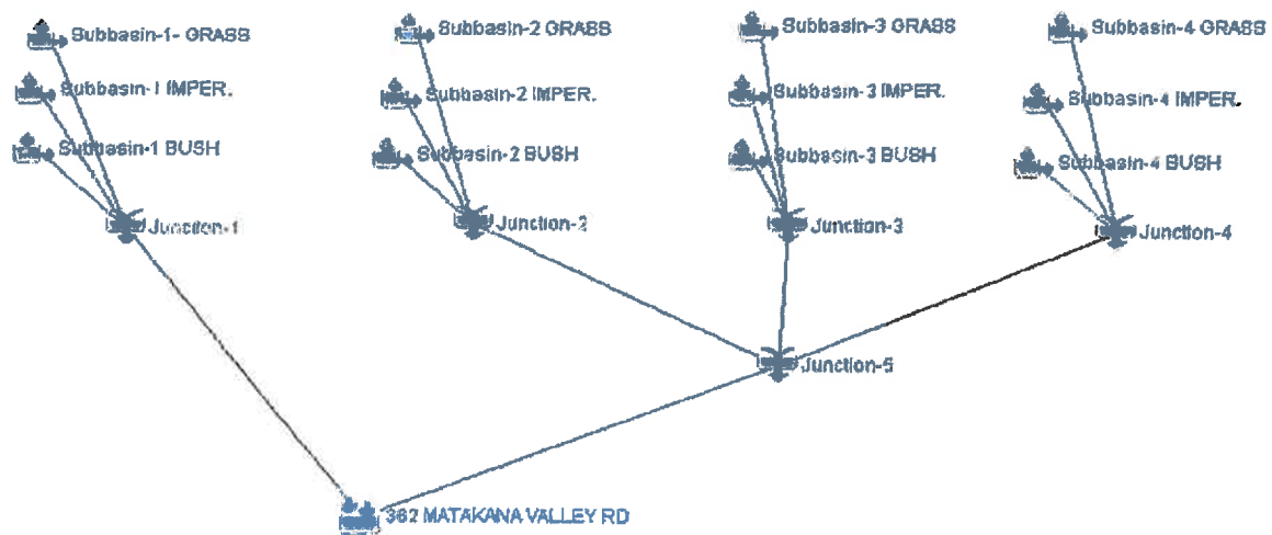
Basin model from HEC HMS
