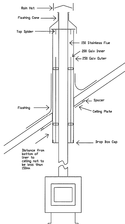
Sloping Ceiling Diagram
