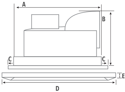
Dimensions - WhisperVent 150
