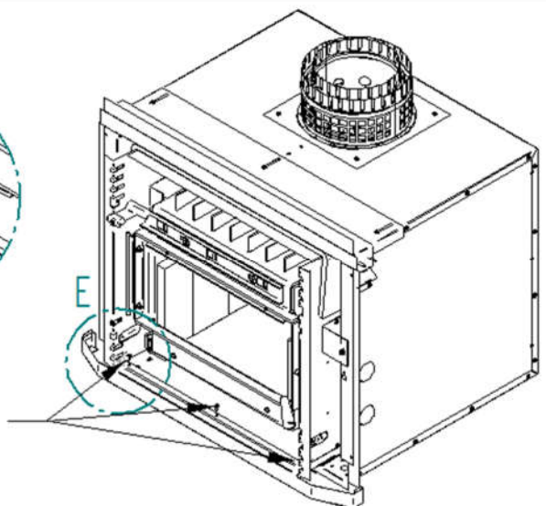
Fig. 20 – Additional Fascia Bottom Piece for ZC
